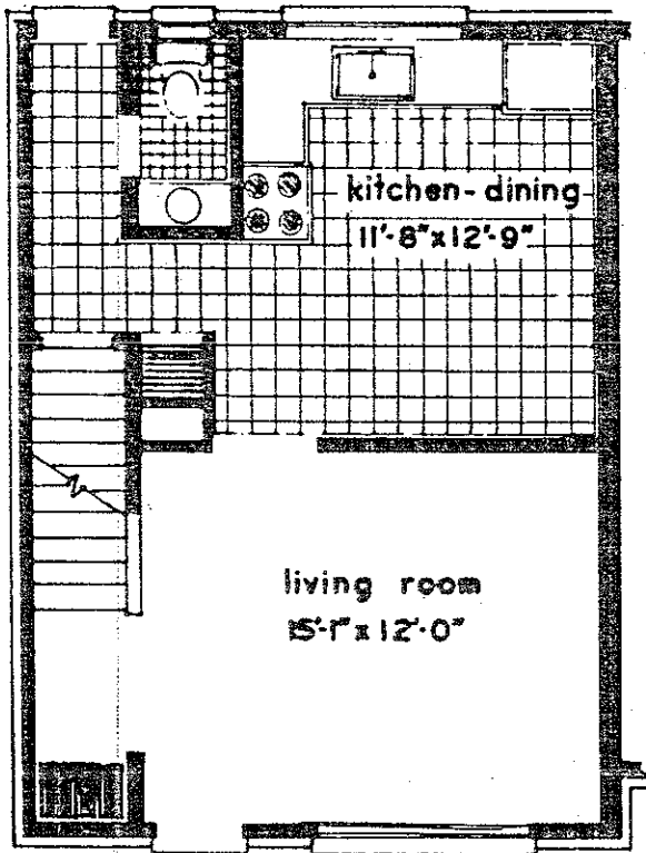
FIRST FLOOR PLAN UNIT "E"
